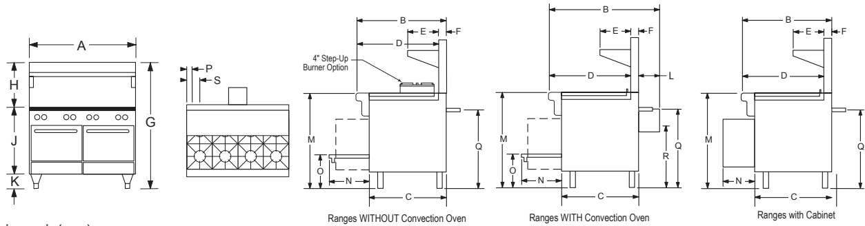
Dimensions - in(mm)
