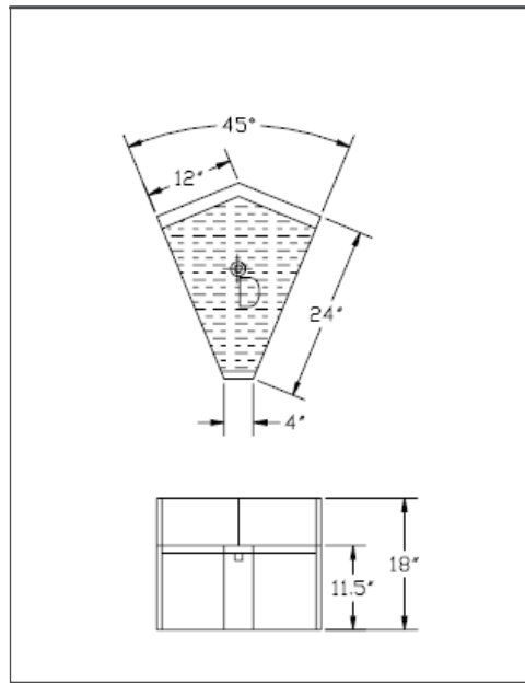
1800 SERIES: KR18-DRC45
