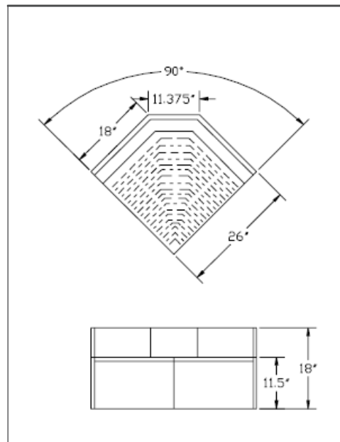
2100 SERIES: KR21-DRC90
