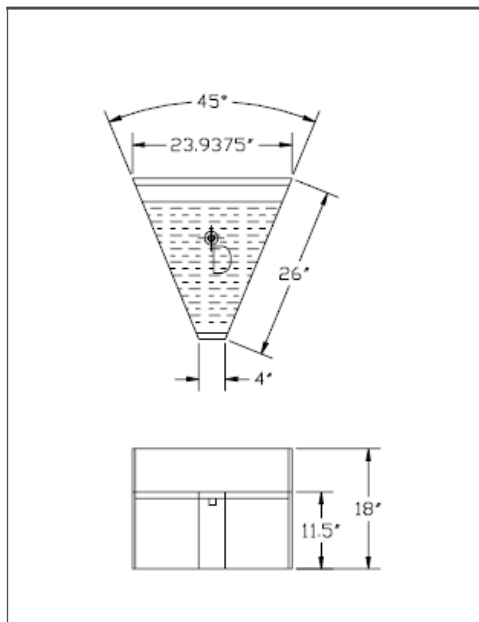
2100 SERIES: KR21-DR45
