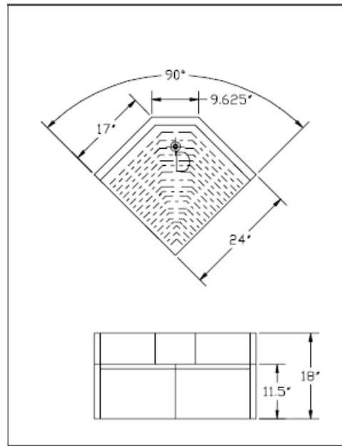
1800 SERIES: KR18-DRC90
