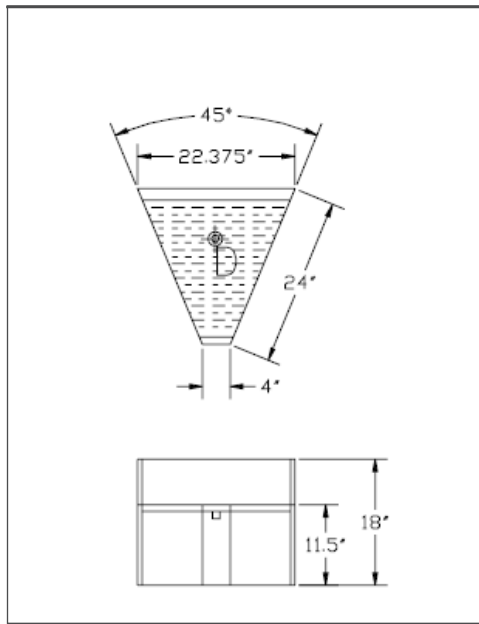
1800 SERIES: KR18-DR45
