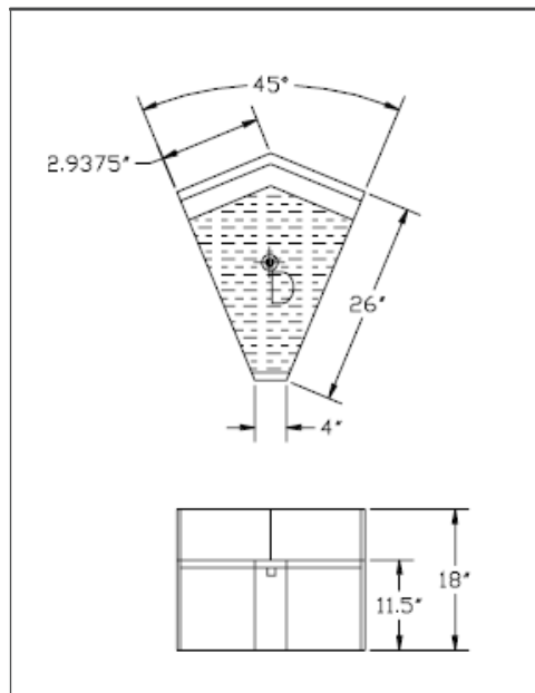
2100 SERIES: KR21-DRC45
