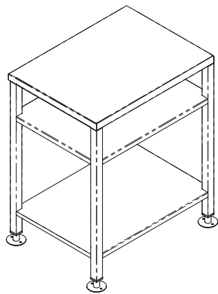
5014986 Stationary with Double Shelf
