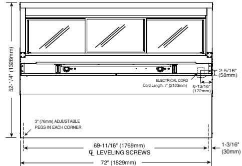
HN2SYS-72 (STANDARD HEIGHT BASE SHOWN)
