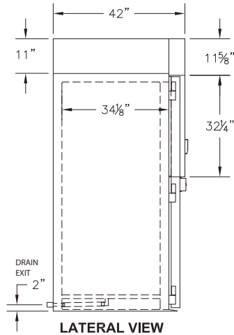
LATERAL VIEW
