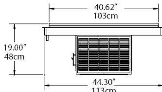
Elevation View
