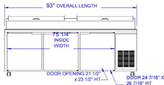
DP93 FRONT VIEW
