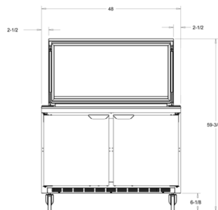
SPE48-18M-STL FRONT VIEW WITH LID OPEN
