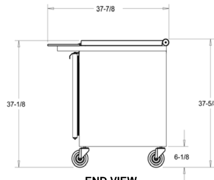
END VIEW WITH LID CLOSED
