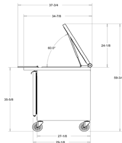
END VIEW WITH LID OPEN
