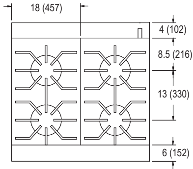
TOP VIEW - 18" OPEN TOP BURNERS
