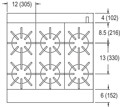
TOP VIEW - 12" OPEN TOP BURNERS
