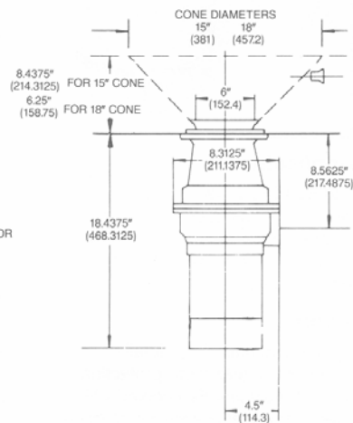
TYPICAL INSTALLATION
