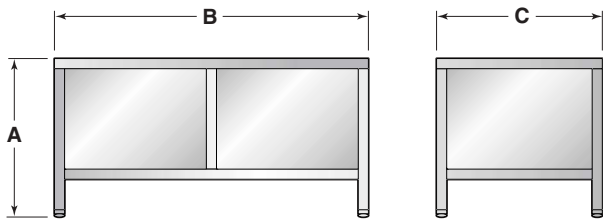
Closed Base Stand
