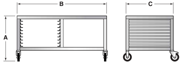
Open Base Stand with Casters and Racks
