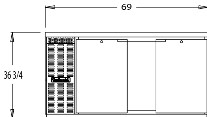
BBC69 FRONT VIEW
