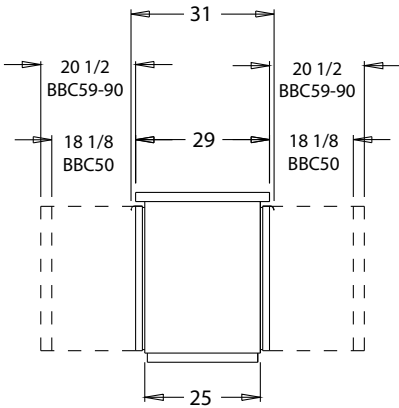
BBC50,59,69,79 & 90 SIDE VIEW
