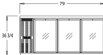
BBC79-GD FRONT VIEW
