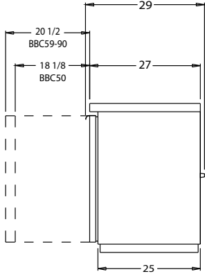
BBC50,59,69,79 & 90 SIDE VIEW
