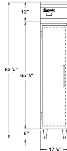
DL1FSES FRONT VIEW
