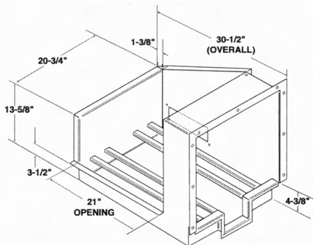
CORNER FEED TABLE STANDARD LEFT P/N 13958.82
