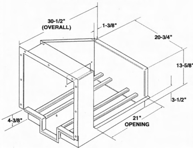
CORNER FEED TABLE STANDARD RIGHT P/N 13958.84
