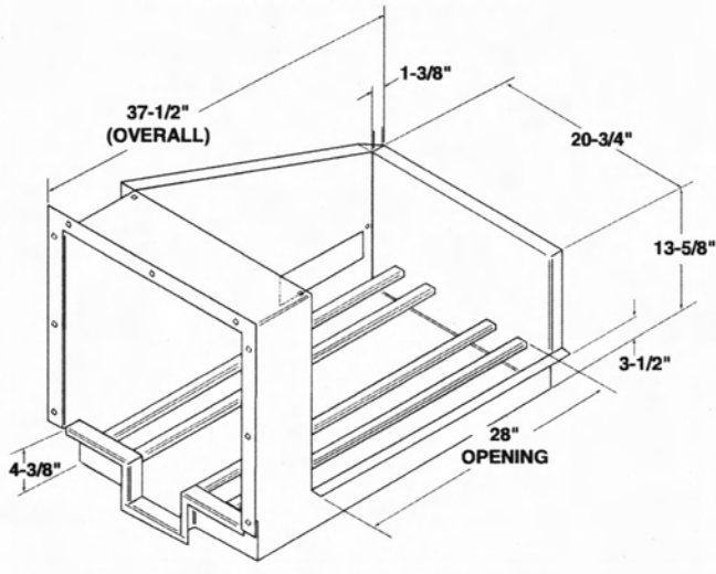
CORNER FEED TABLE SHEET PAN RIGHT P/N 13960.00
