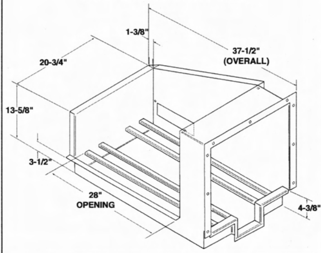
CORNER FEED TABLE SHEET PAN LEFT P/N 13959.00
