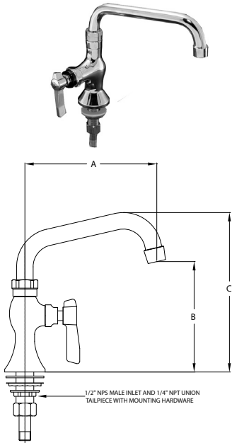
Dimensions shown in inches (mm) are for reference only and are subject to change.
