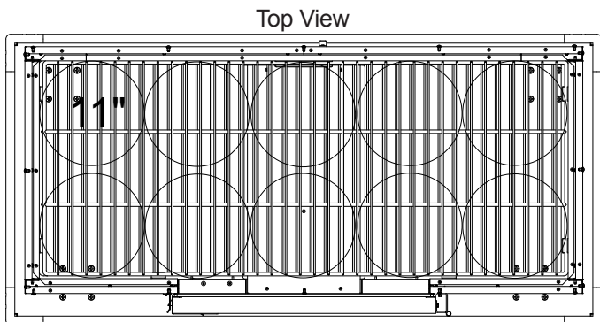
11" Covered Plate Configuration stacked three shelves 5 high.
