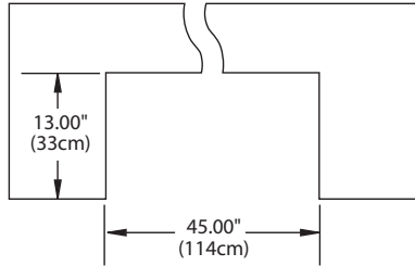
Cutout Dimension
