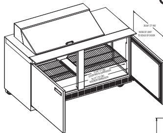
4464N-18M ISO View
