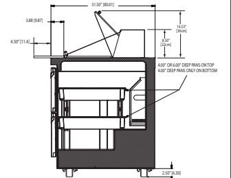
D4464N-12M Right Side View
