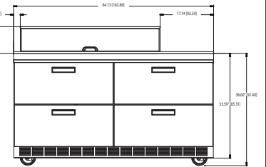
D4464N-18M Elevation View
