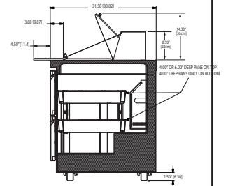
D4464N-18M Right Side View
