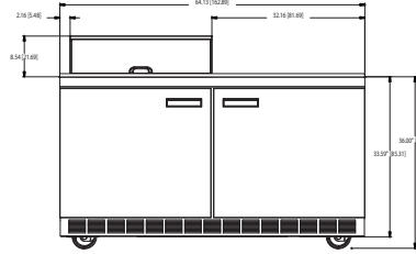
4464N-12M Elevation View
