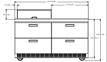
D4464N-12M Elevation View
