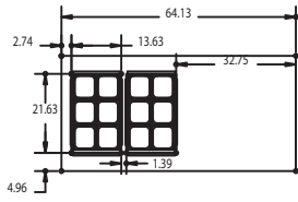
4464N-12M Pan Cutout Configuration
