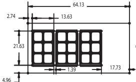
D4464N-18M Pan Cutout Configuration
