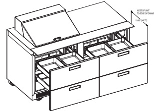
D4464N-12M ISO View
