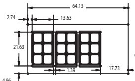
4464N-18M Pan Cutout Configuration
