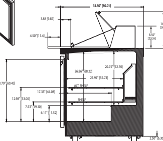
4464N-18M Right Side View
