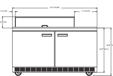
4464N-18M Elevation View
