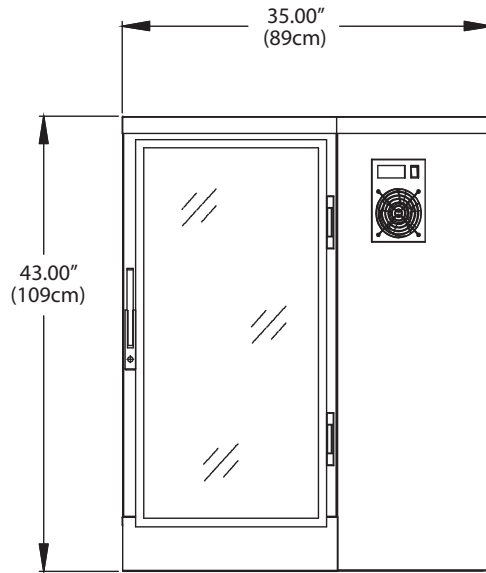
Elevation View HDR316
