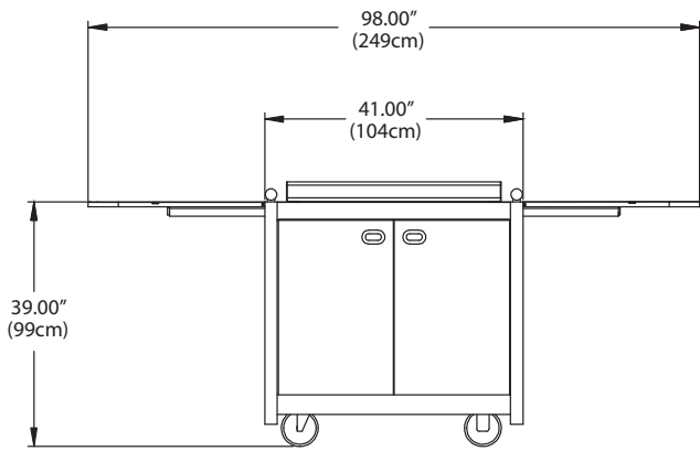
Elevation View
