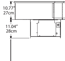
N8194-BR Side View
