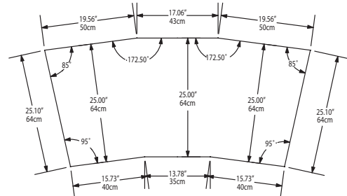
N8159-BR Cutout Dimensions
