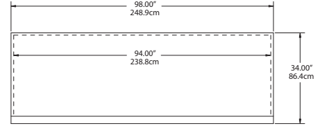
PLAN VIEW SSRR13-G, SARR13-G, SMRR13-G
