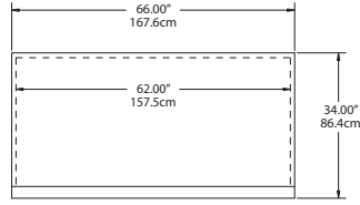
PLAN VIEW SSRR12-G, SARR12-G, SMRR12-G
