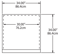
PLAN VIEW SSRR11-G, SARR11-G, SMRR11-G
