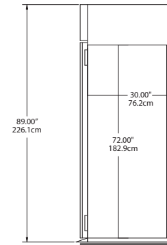
END VIEW ALL MODELS
