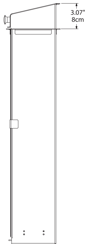
Right End View SB-1
