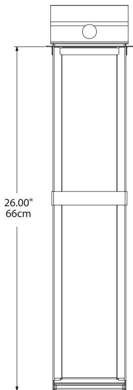
Elevation View SB-1
