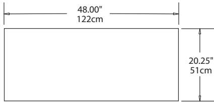
Plan View SCN-48
