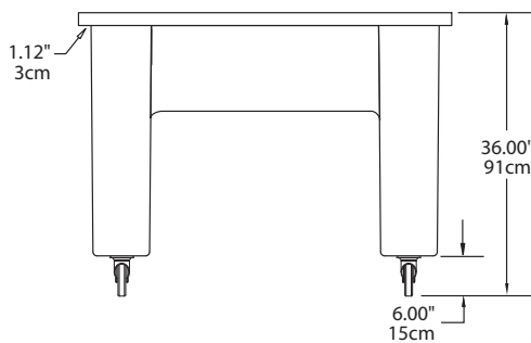
Elevation View SCN-48
