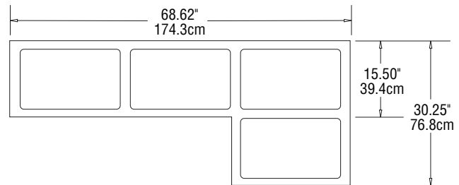
PLAN VIEW SLT4-R
