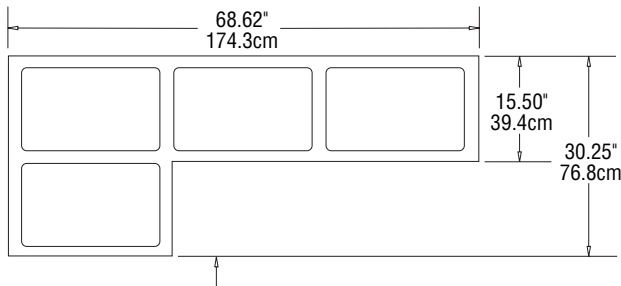
PLAN VIEW SLT4-L
