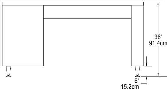
ELEVATION VIEW SLT4-L
