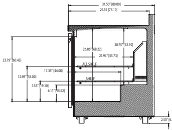
ST4464N Right Side View
