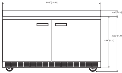
ST4464N Elevation View
