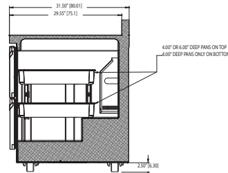
STD4464N Right Side View
