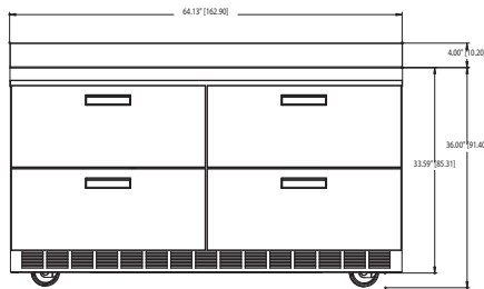
STD4464N Elevation View
