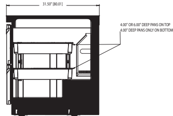
UCD4464N Right Side View
