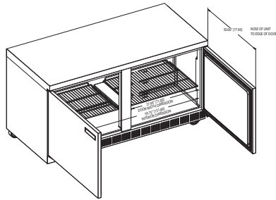
UC4464N ISO View
