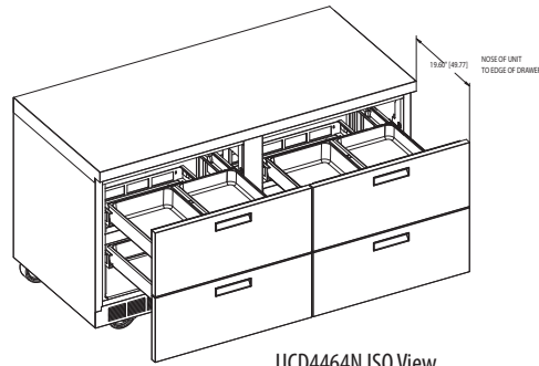
UCD4464N ISO View
