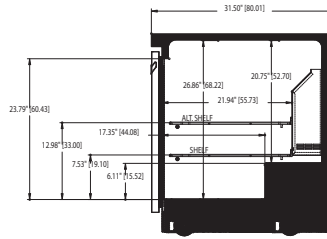
UC4464N Right Side View
