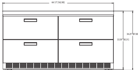
UCD4464N Elevation View
