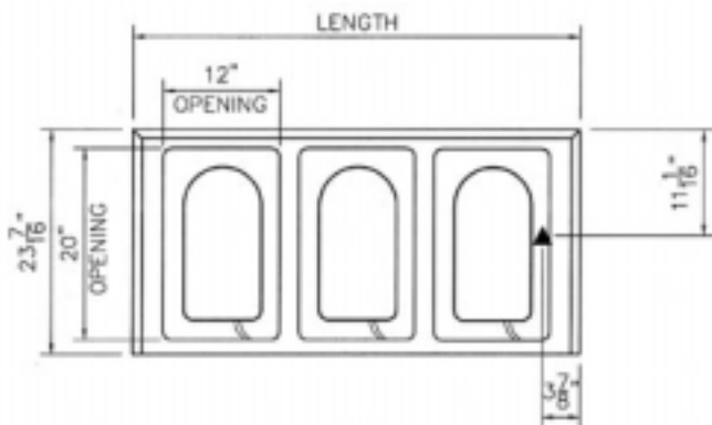
ASI-3E UNIT SHOWN TOP VIEW
