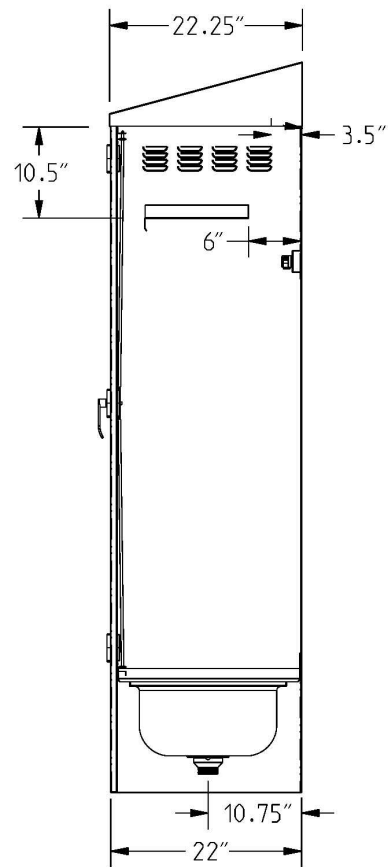
SIDE VIEW (section)
