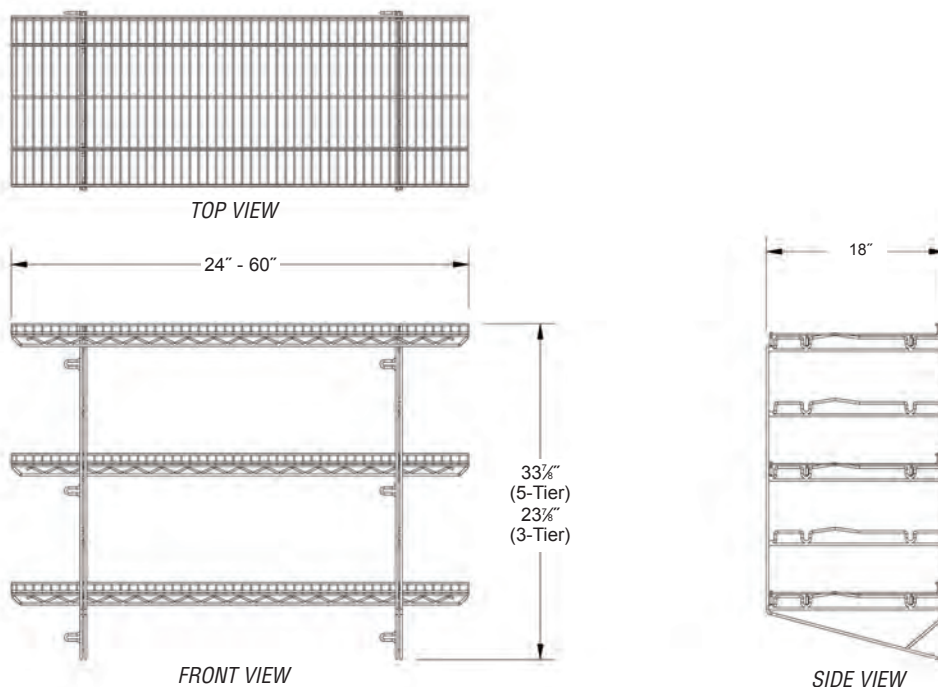
(5-tier bracket kit shown with 3 shelves - S3-5B-SSW1848C)
