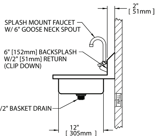
BACKSPLASH DETAIL
