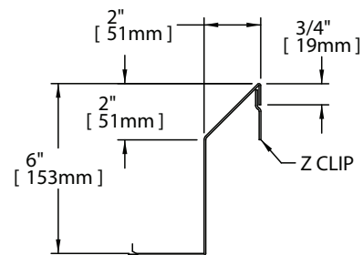
BACKSPLASH DETAIL
