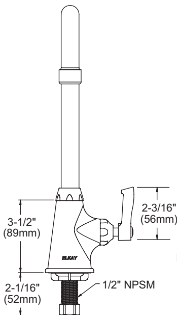
Model LK535GN04L2 FRONT VIEW
