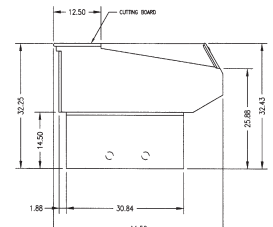
SIDE VIEW Self-Serve Case
