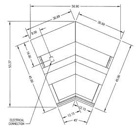
TOP VIEW SQRIC45SSR
