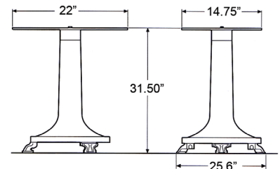
Pedestal for 250VO and 300VO
