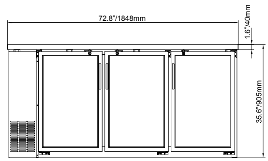
73-inch 3 doors bottle cooler Item: 37549 Model: BB-CN-0020-S
