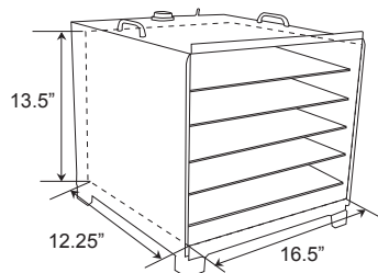
INNER DIMENSIONS
