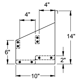
SIDE ELEVATION
