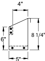
SIDE ELEVATION
