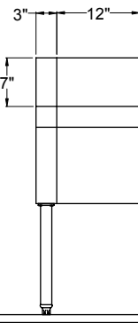
FRONT ELEVATION
