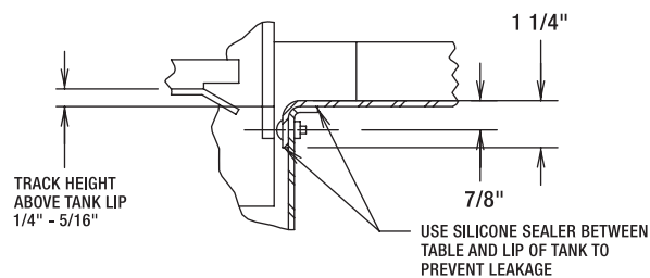
SECTIONAL VIEW SHOWING TABLE CONNECTIONS
