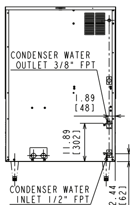
WATER-COOLED UNIT BACK VIEW
