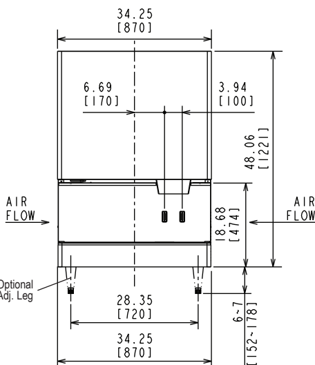
AIR-COOLED UNIT FRONT VIEW
