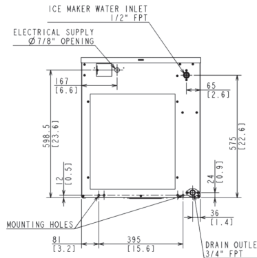
AIR-COOLED UNIT
