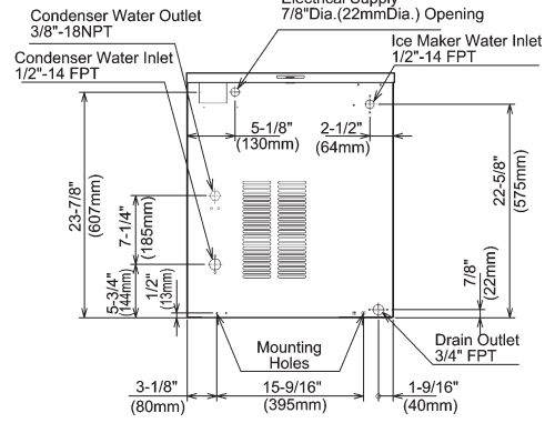
WATER-COOLED UNIT
