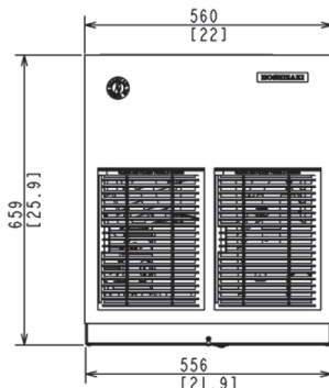
FRONT VIEW (Air)
