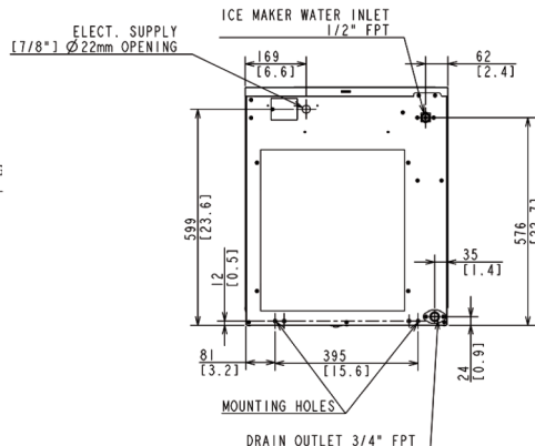
AIR-COOLED UNIT
