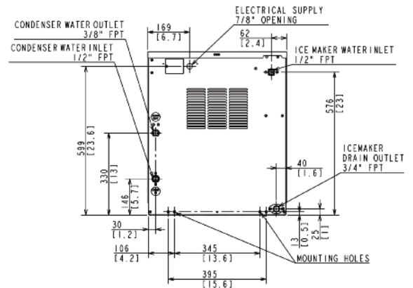
WATER-COOLED UNIT
