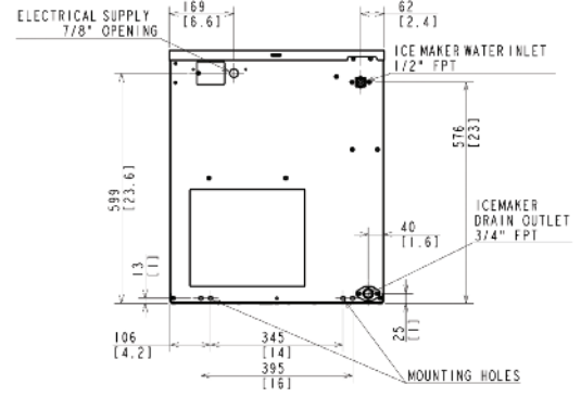
AIR-COOLED UNIT
