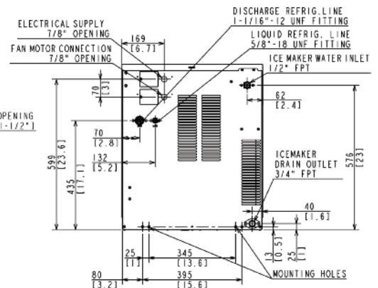
REMOTE AIR-COOLED UNIT
