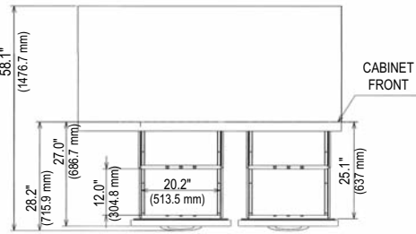
HUR68A-D (TOP VIEW)
