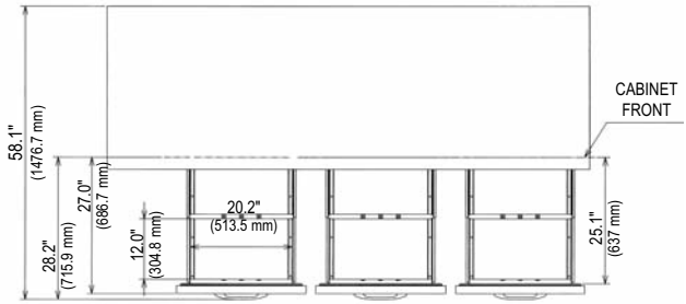
HUR96A-D (TOP VIEW)
