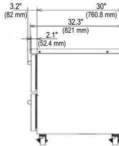
SIDE VIEW (ALL UNITS)
