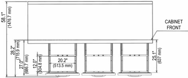
HWR96A-D (TOP VIEW)
