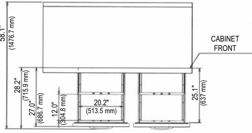
HWR68A-D (TOP VIEW)
