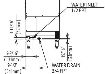
BACK VIEW - AIR-COOLED UNIT
